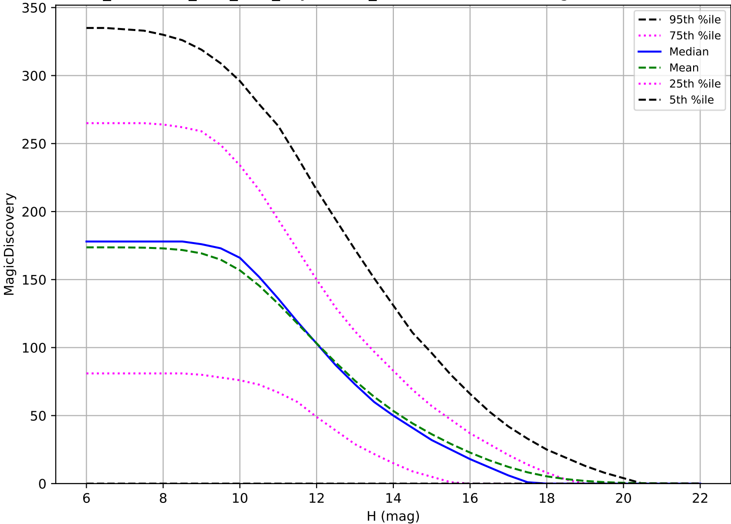
too_combined_s1.0_v3.4_10yrs: OCC_r5 6 detections in 60 nights detection loss
