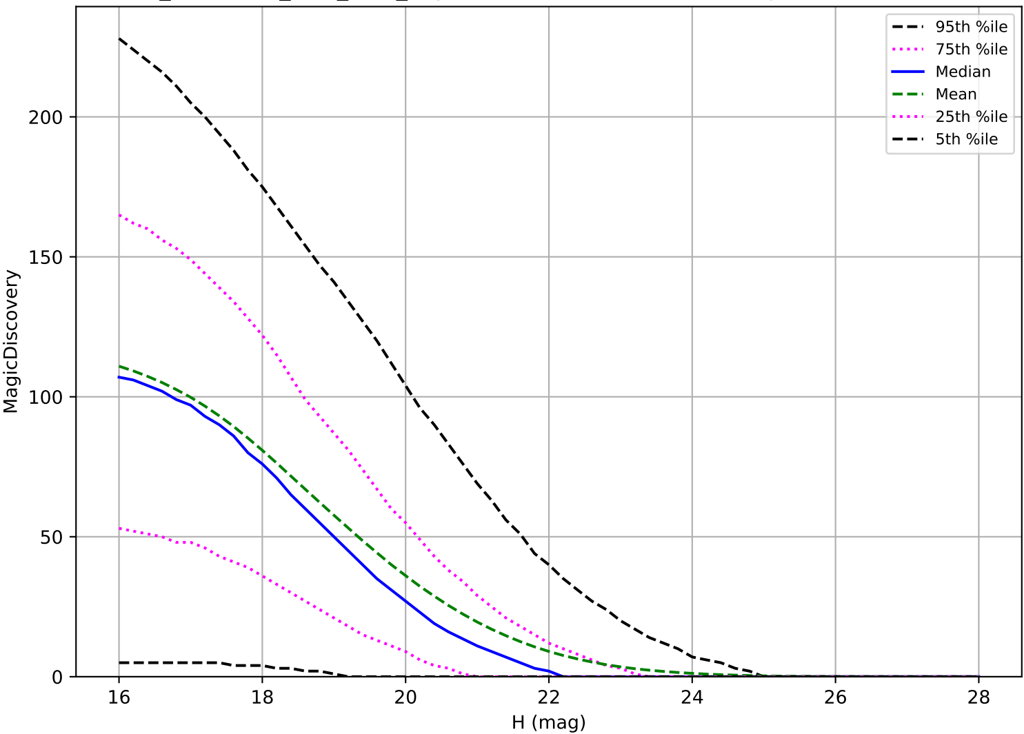
too_combined_s1.0_v3.4_10yrs: NEO 6 detections in 60 nights detection loss
