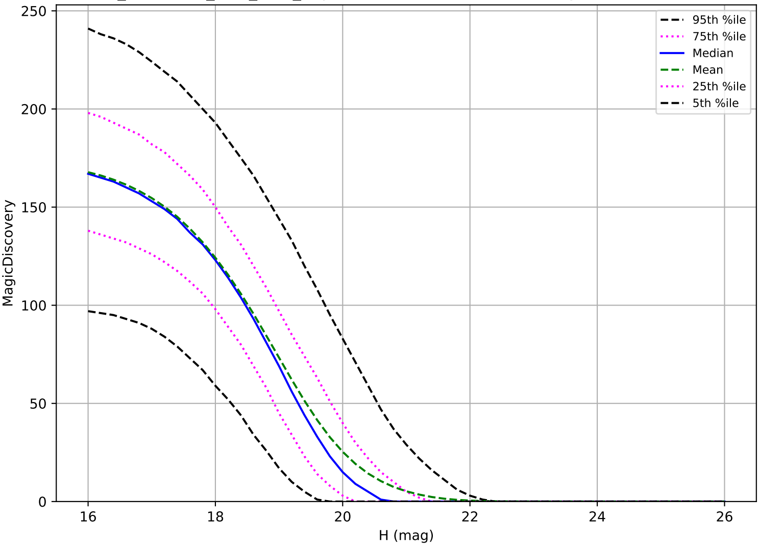
too_combined_s1.0_v3.4_10yrs: MBA 6 detections in 60 nights detection loss
