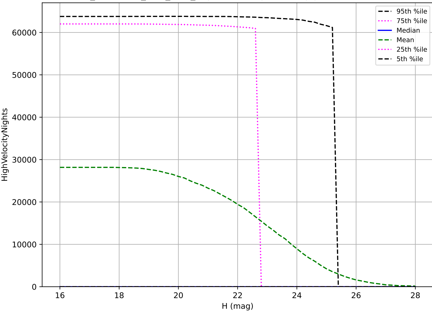
too_combined_s1.0_v3.4_10yrs: PHA High velocity pair detection loss
