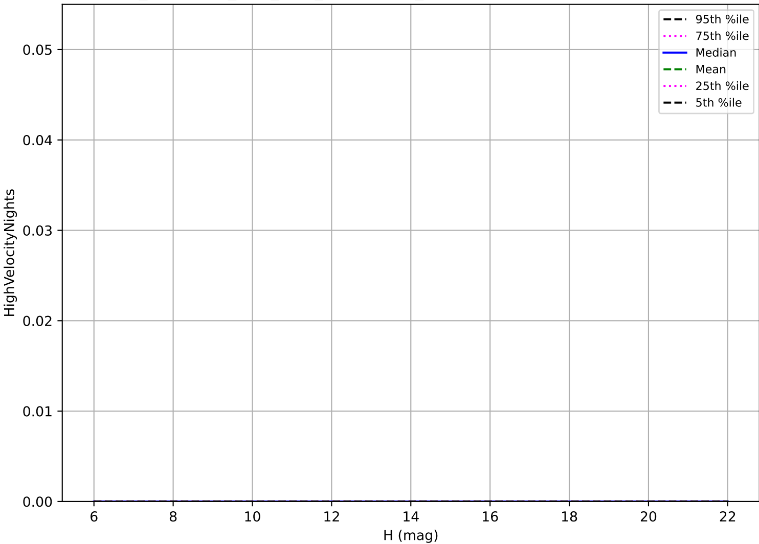
too_combined_s1.0_v3.4_10yrs: OCC_r5 High velocity pair detection loss
