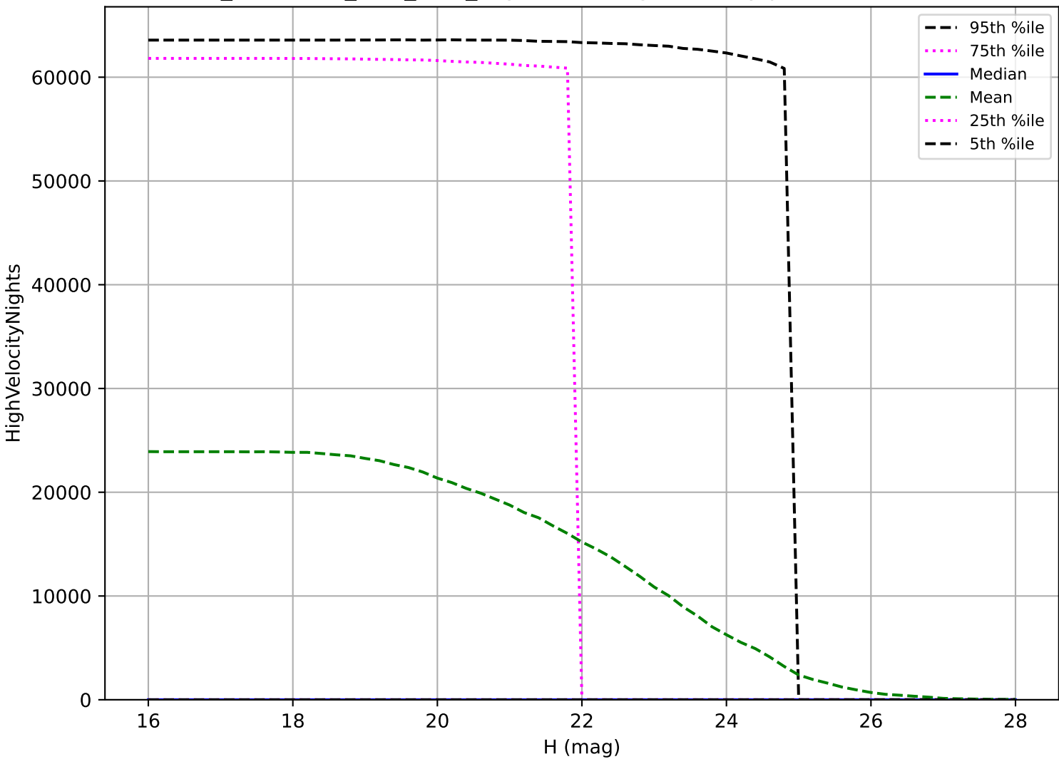
too_combined_s1.0_v3.4_10yrs: NEO High velocity pair detection loss
