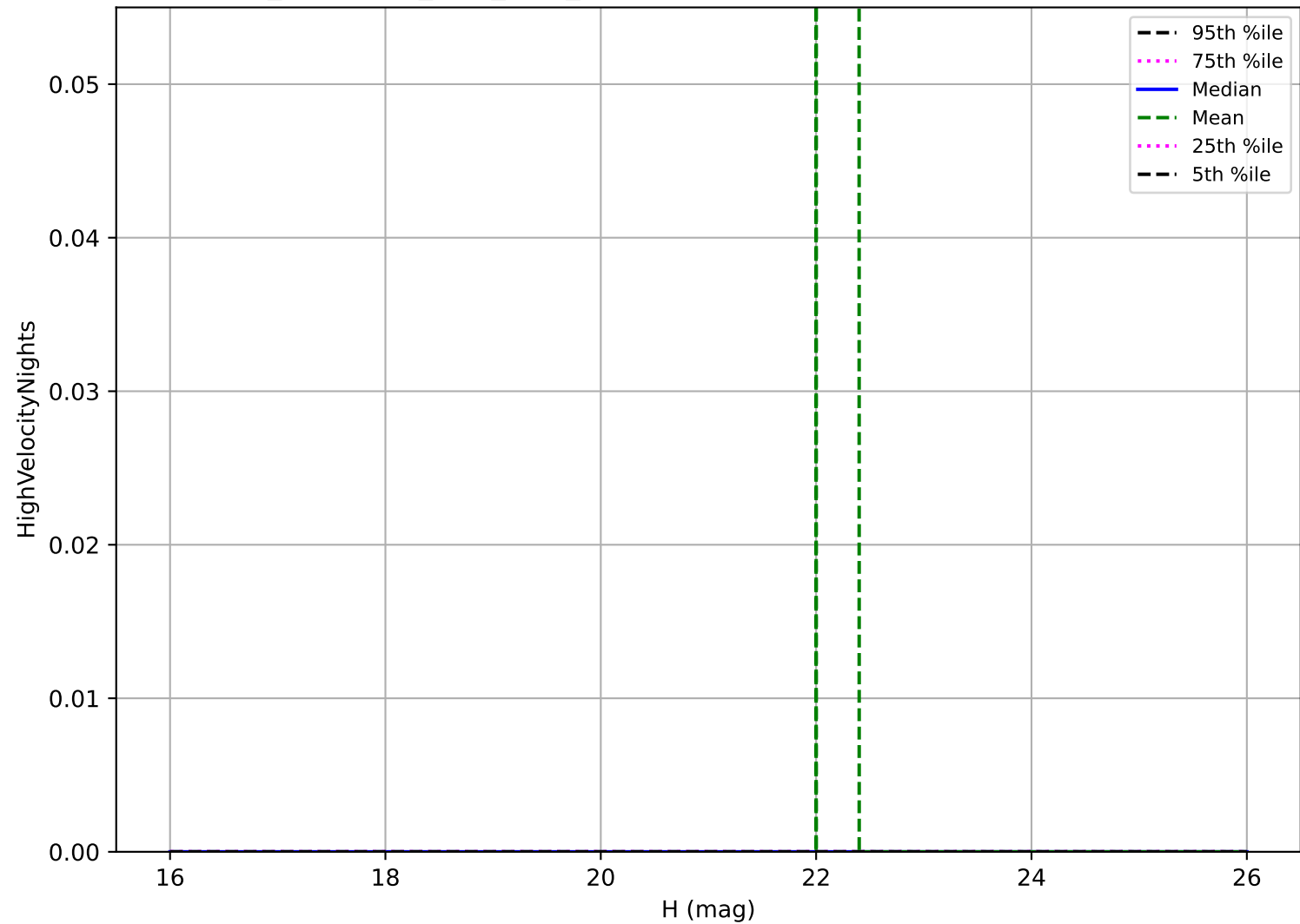
too_combined_s1.0_v3.4_10yrs: MBA High velocity pair detection loss
