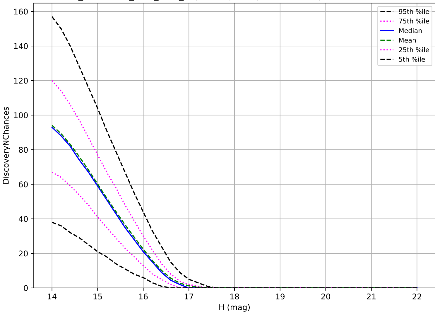
too_combined_s1.0_v3.4_10yrs: Trojan 3 pairs in 15 nights detection loss
