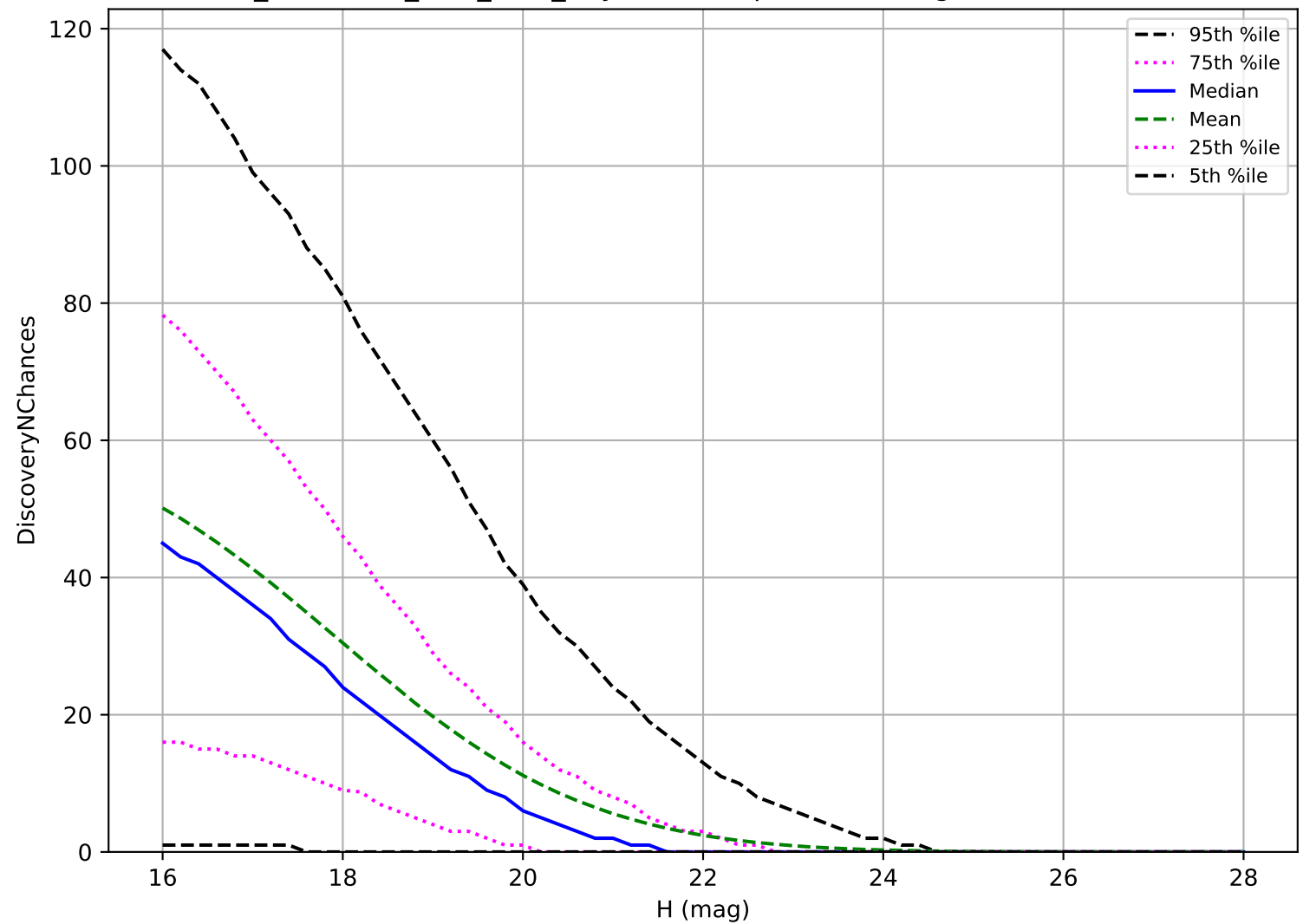
too_combined_s1.0_v3.4_10yrs: PHA 3 pairs in 15 nights detection loss
