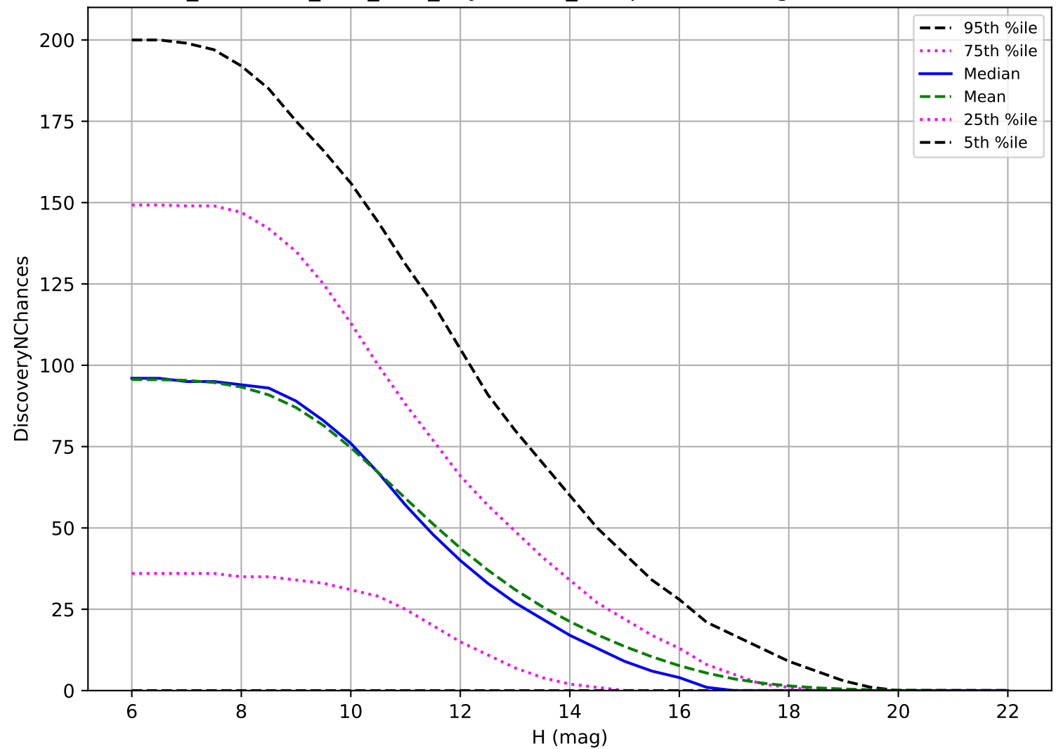
too_combined_s1.0_v3.4_10yrs: OCC_r5 3 pairs in 15 nights detection loss
