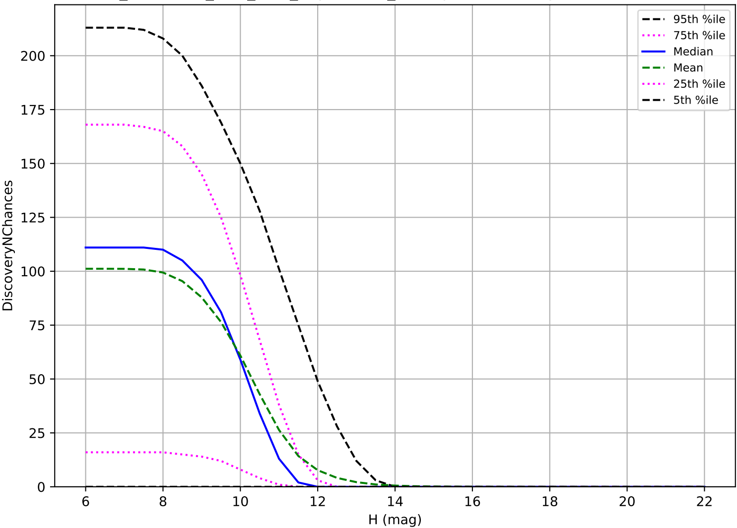
too_combined_s1.0_v3.4_10yrs: OCC_r20 3 pairs in 15 nights detection loss
