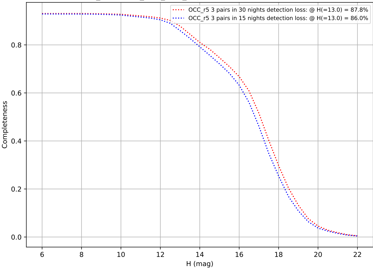
too_combined_s1.0_v3.4_10yrs: DifferentialCompleteness
