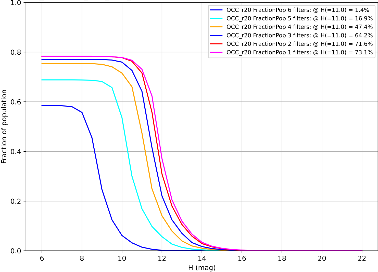
too_combined_s1.0_v3.4_10yrs: Fraction of population with colors in X filters OCC_r20
