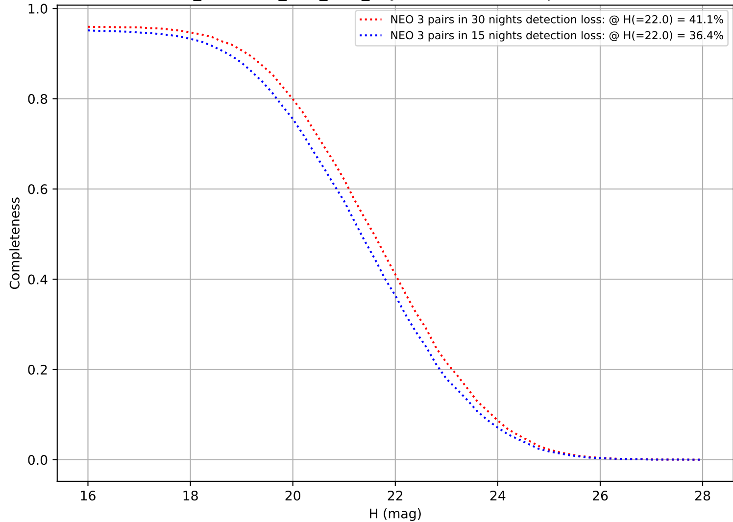
too_combined_s1.0_v3.4_10yrs: DifferentialCompleteness
