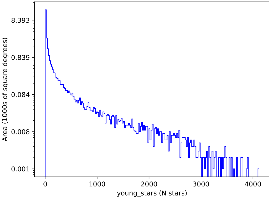
too_combined_s1.0_v3.4_10yrs : young_stars
