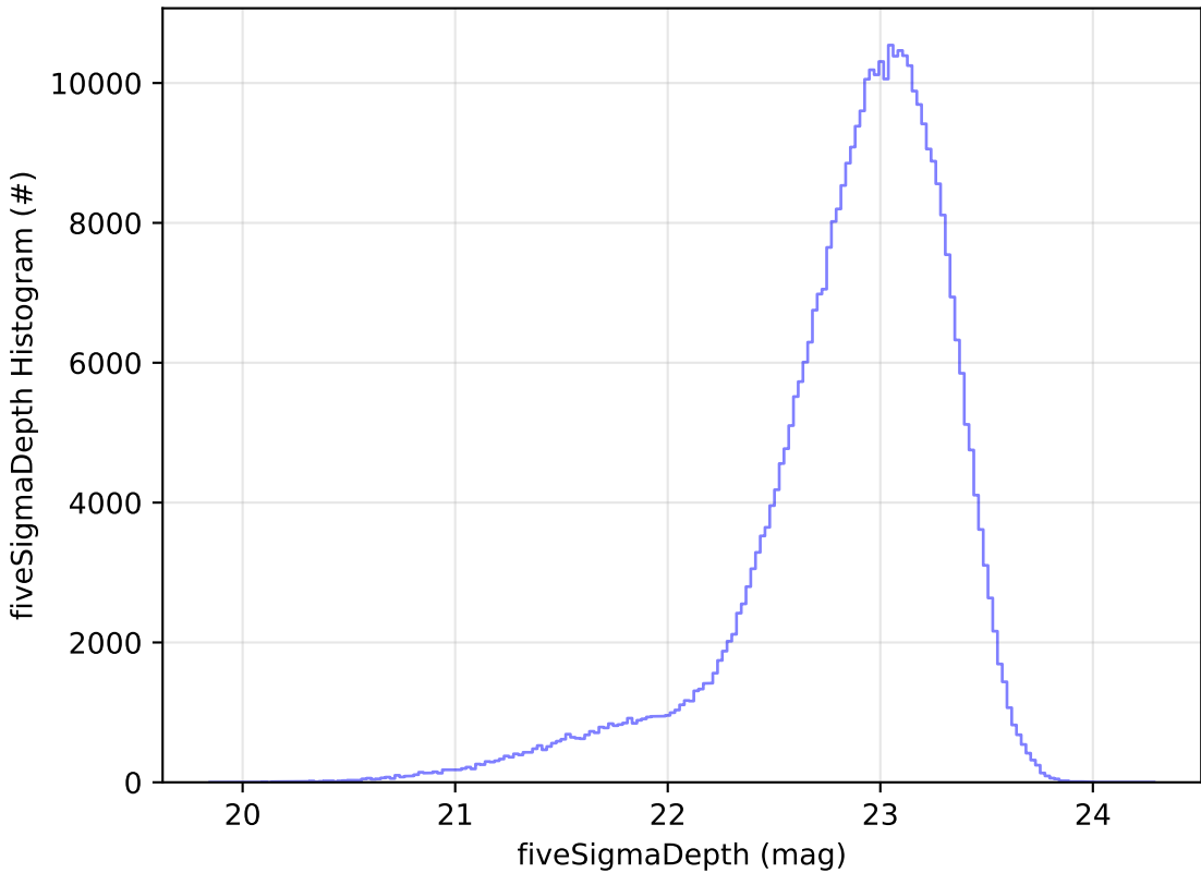
too_combined_s1.0_v3.4_10yrs z: fiveSigmaDepth Histogram
