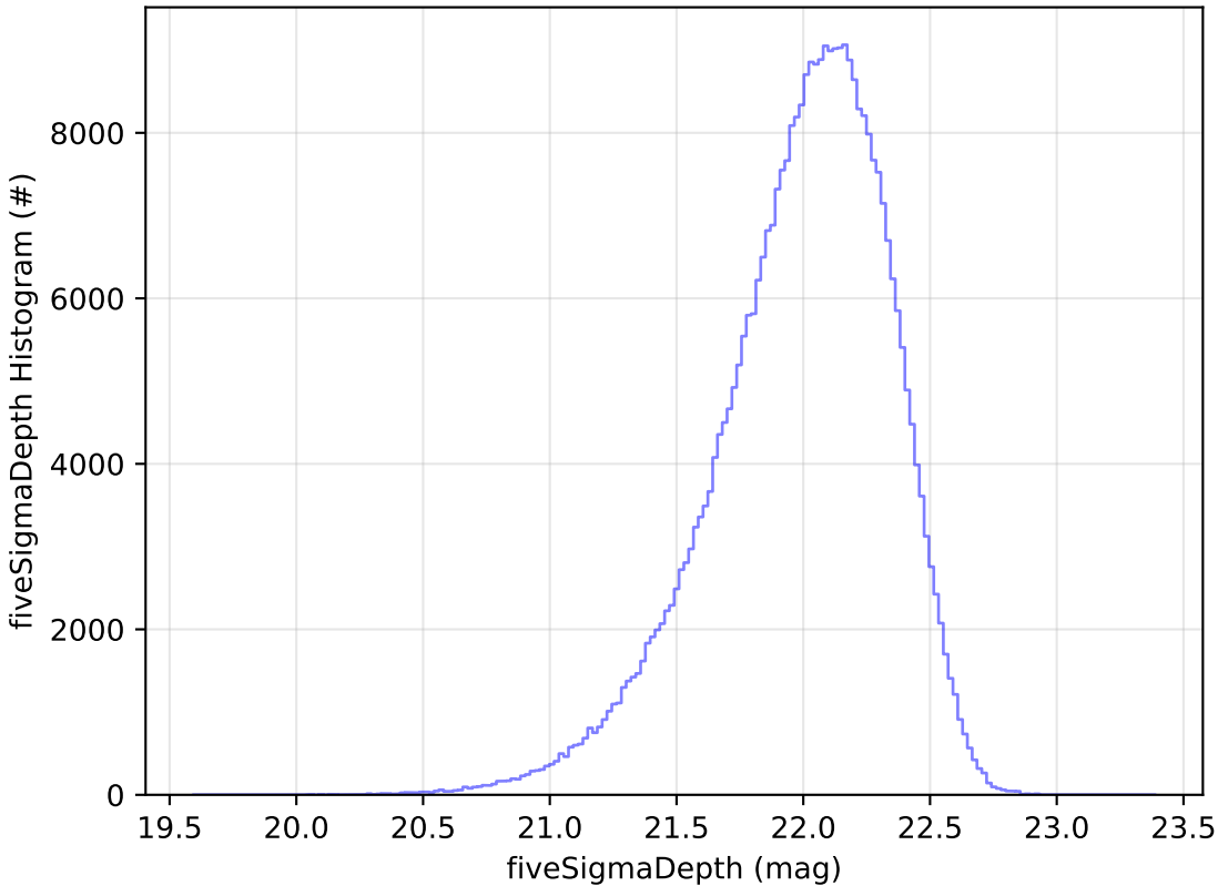
too_combined_s1.0_v3.4_10yrs y: fiveSigmaDepth Histogram
