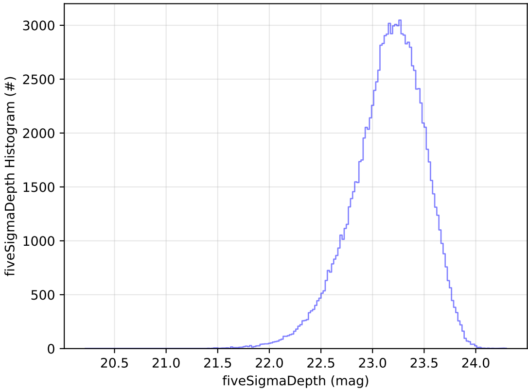
too_combined_s1.0_v3.4_10yrs u: fiveSigmaDepth Histogram
