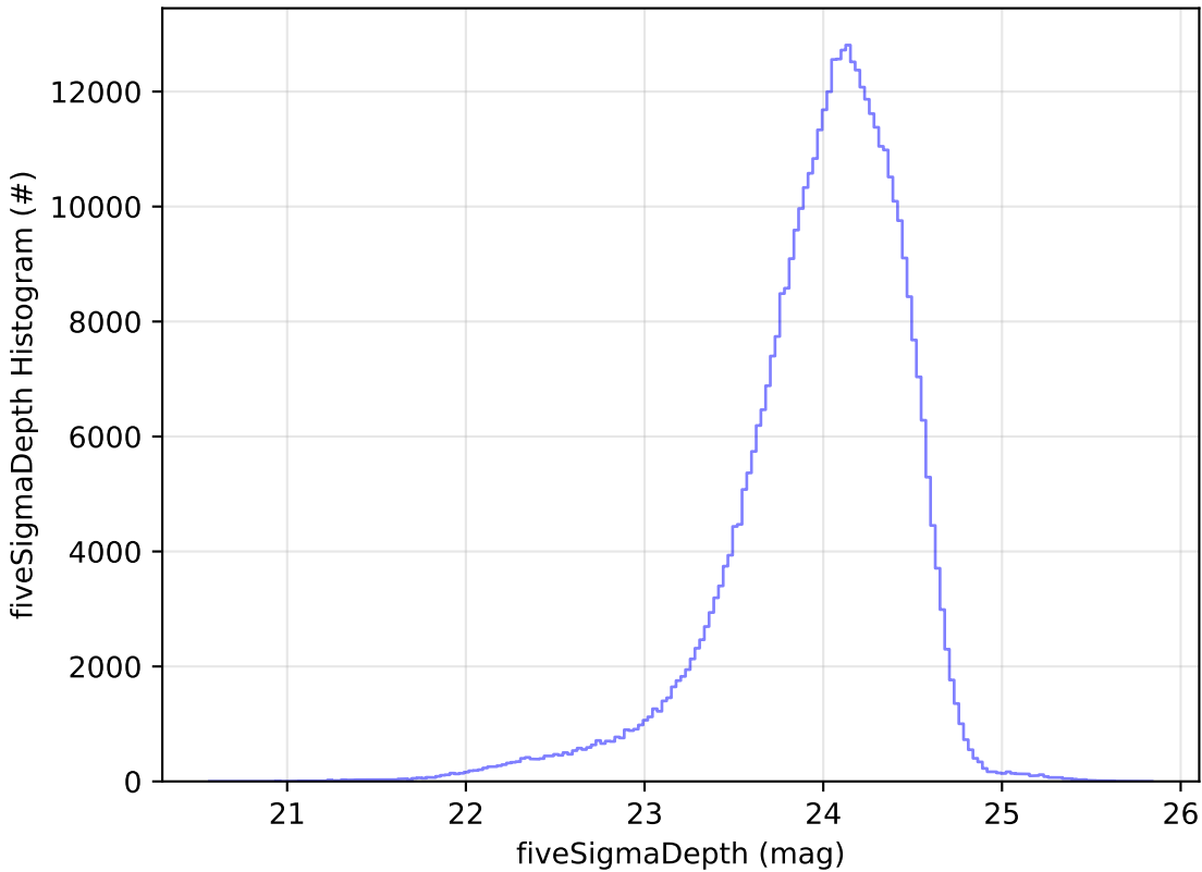
too_combined_s1.0_v3.4_10yrs r: fiveSigmaDepth Histogram
