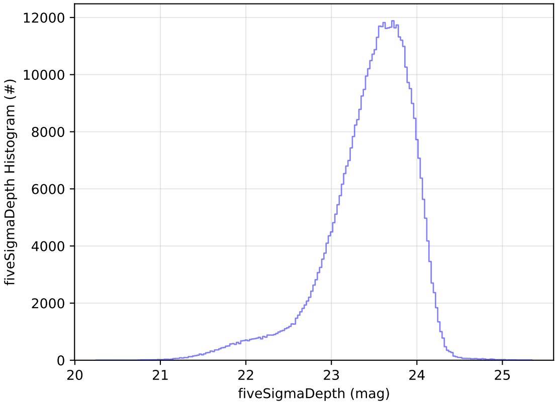
too_combined_s1.0_v3.4_10yrs i: fiveSigmaDepth Histogram
