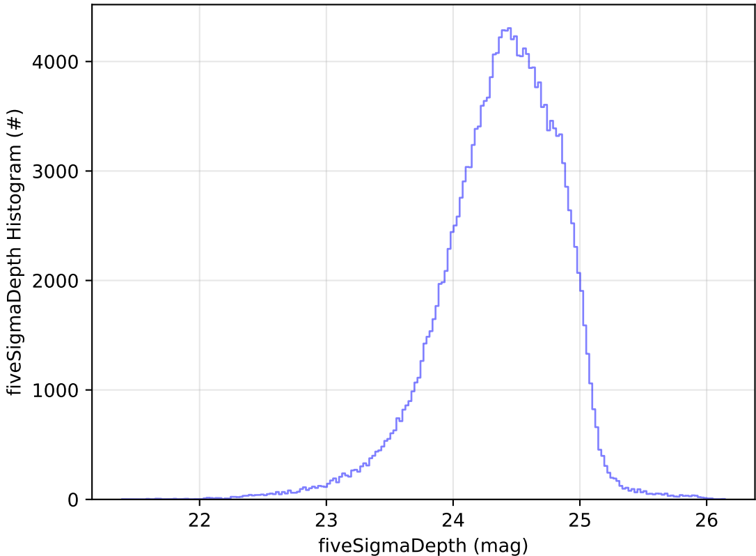
too_combined_s1.0_v3.4_10yrs g: fiveSigmaDepth Histogram
