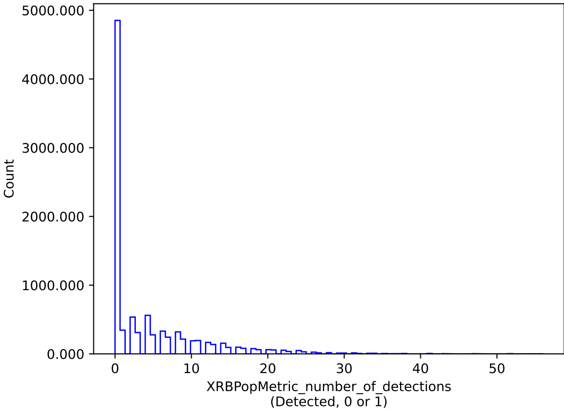
too_combined_s1.0_v3.4_10yrs : XRBPoMetric_number_of_detections
