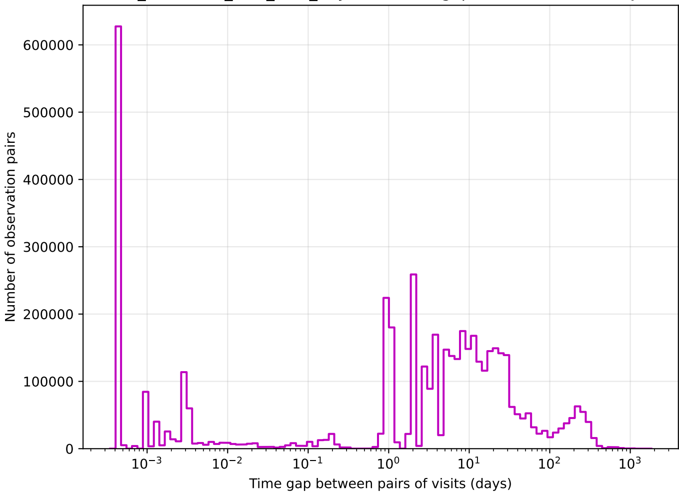
too_combined_s1.0_v3.4_10yrs z band: Tgaps observationStartMJD
