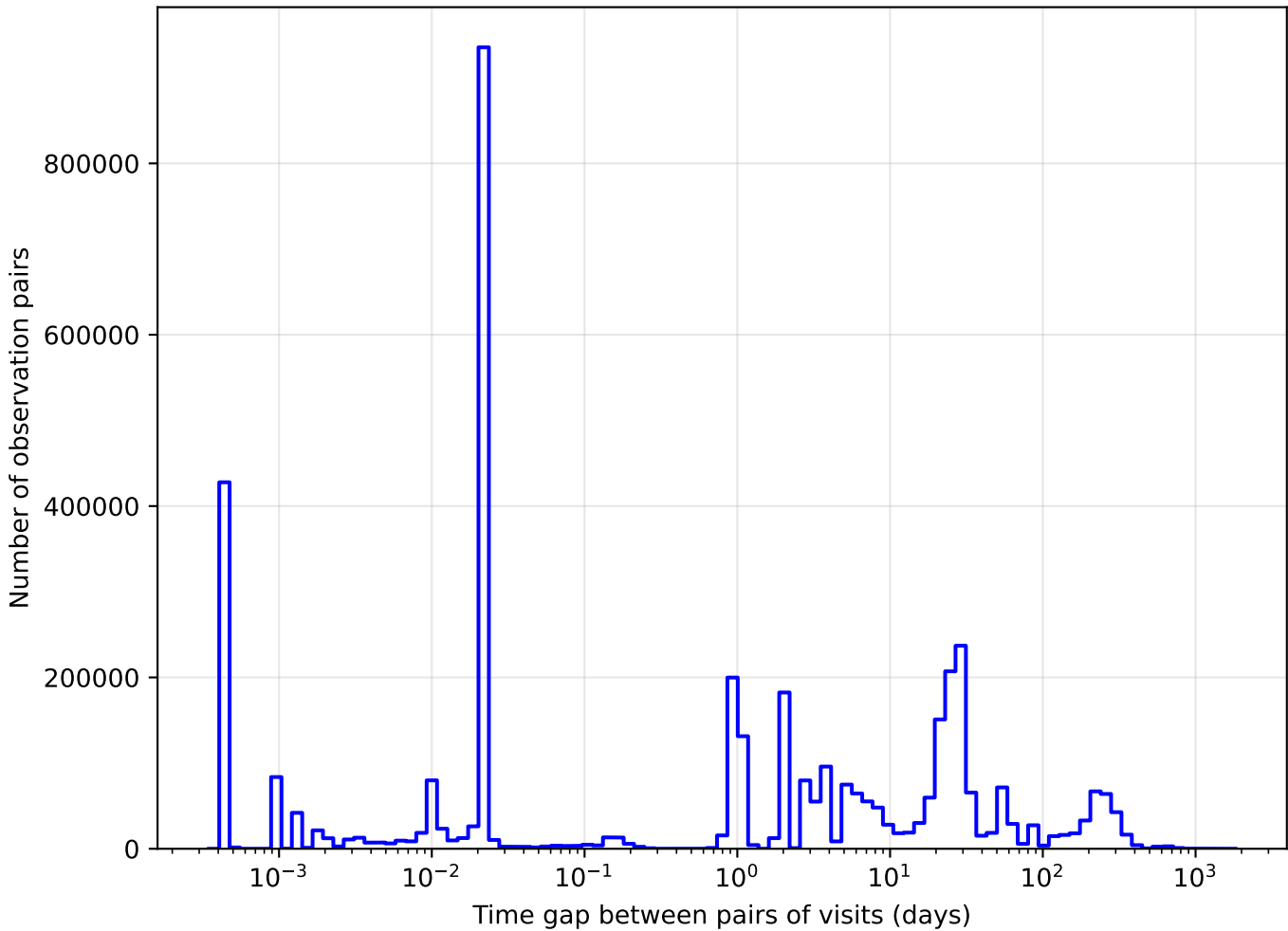
too_combined_s1.0_v3.4_10yrs y band: Tgaps observationStartMJD
