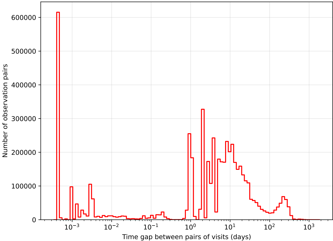
too_combined_s1.0_v3.4_10yrs i band: Tgaps observationStartMJD
