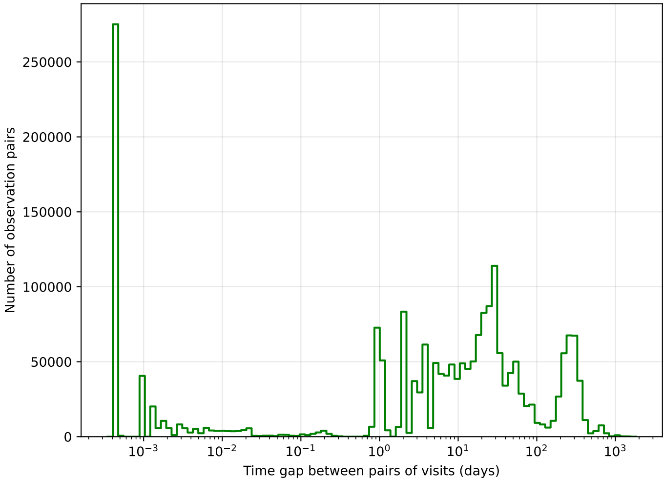
too_combined_s1.0_v3.4_10yrs g band: Tgaps observationStartMJD
