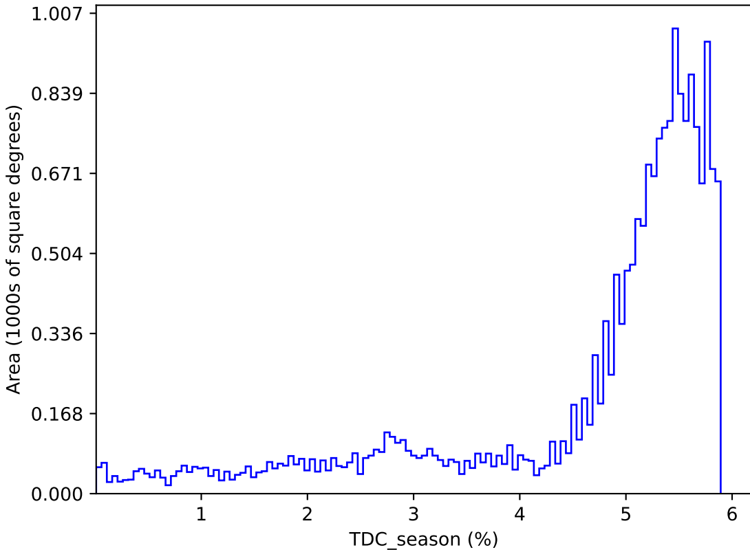
too_combined_s1.0_v3.4_10yrs : TDC_season
