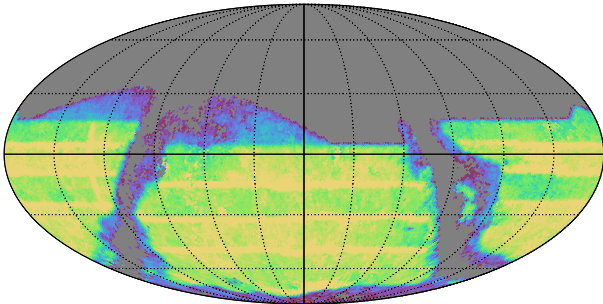
too_combined_s1.0_v3.4_10yrs : TDC_rate
