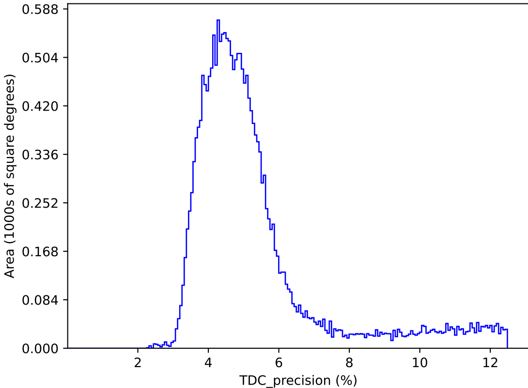
too_combined_s1.0_v3.4_10yrs : TDC_precision
