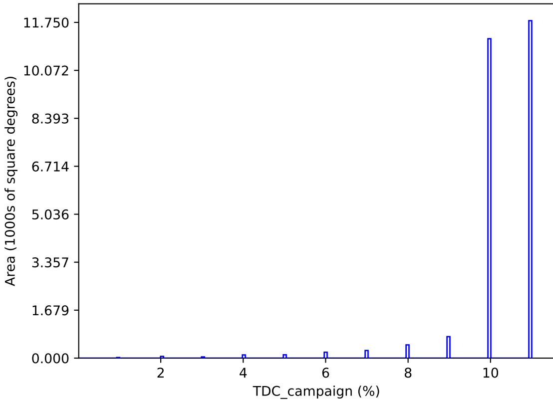
too_combined_s1.0_v3.4_10yrs : TDC_campaign
