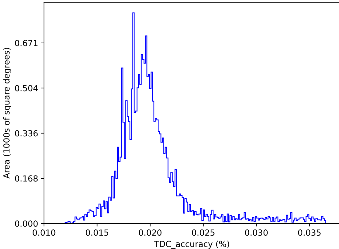
too_combined_s1.0_v3.4_10yrs : TDC_accuracy
