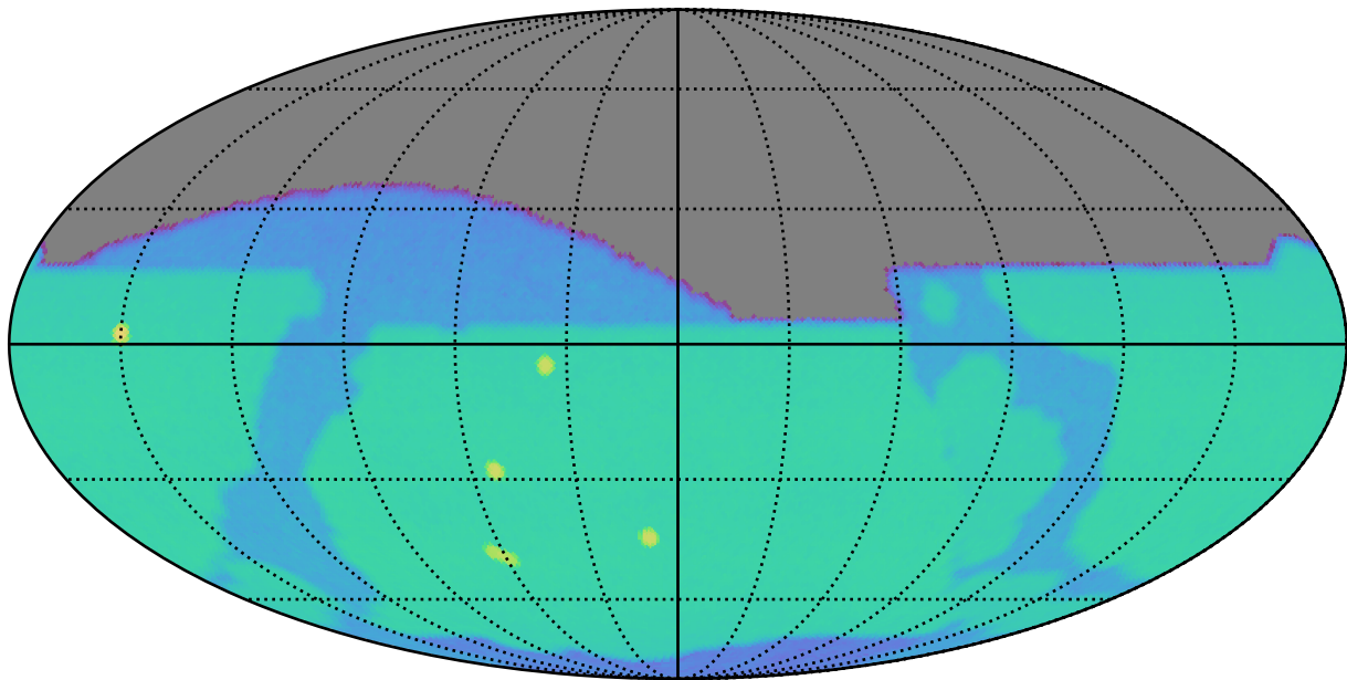
too_combined_s1.0_v3.4_10yrs z: SurfaceBrightLimit
