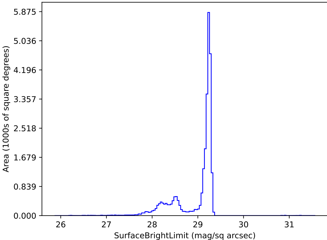
too_combined_s1.0_v3.4_10yrs z: SurfaceBrightLimit
