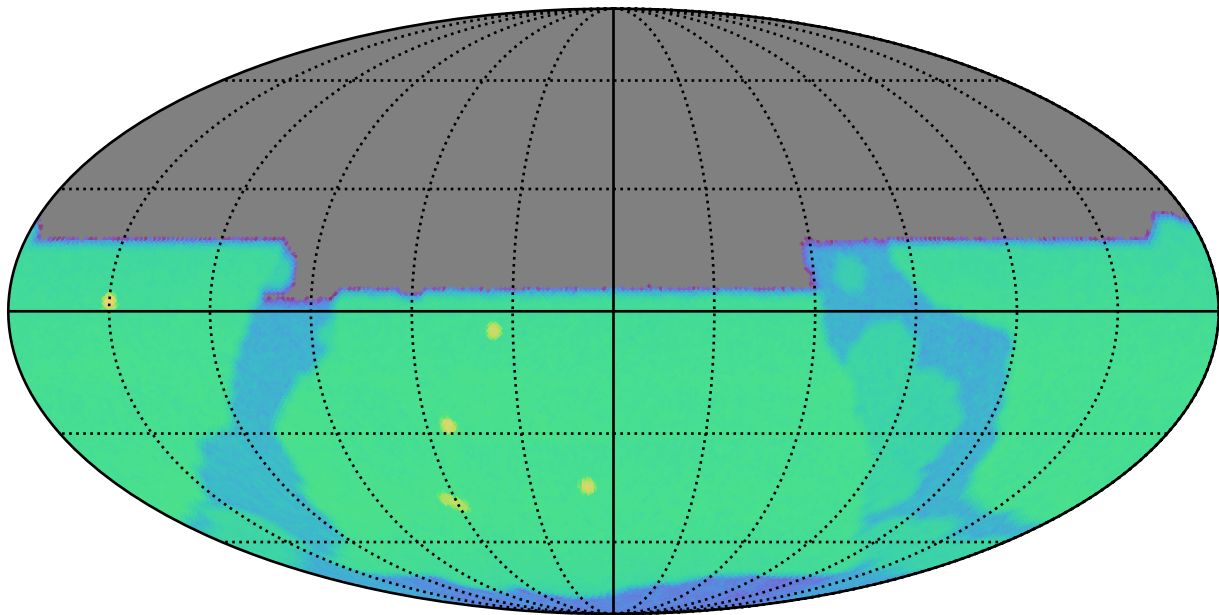
too_combined_s1.0_v3.4_10yrs y: SurfaceBrightLimit
