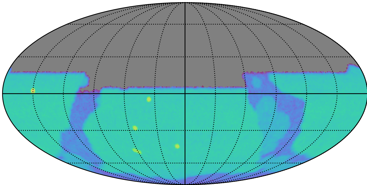
too_combined_s1.0_v3.4_10yrs u: SurfaceBrightLimit
