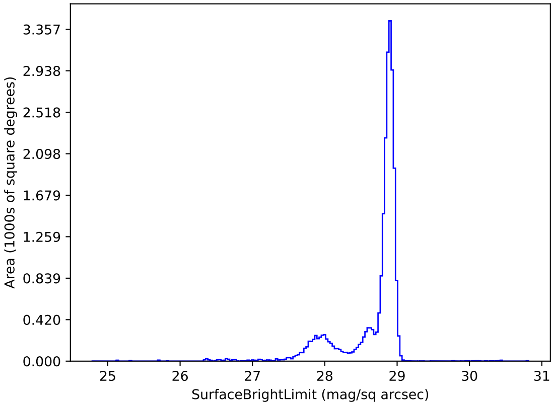
too_combined_s1.0_v3.4_10yrs u: SurfaceBrightLimit
