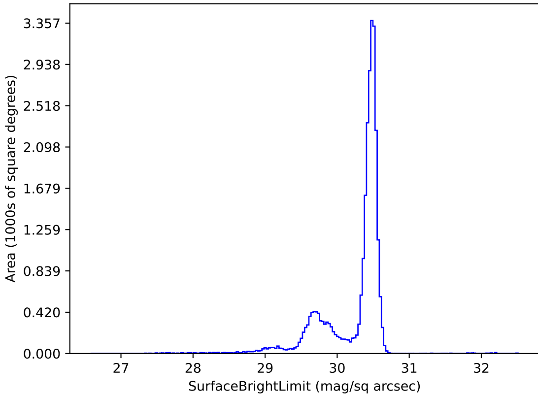
too_combined_s1.0_v3.4_10yrs r: SurfaceBrightLimit
