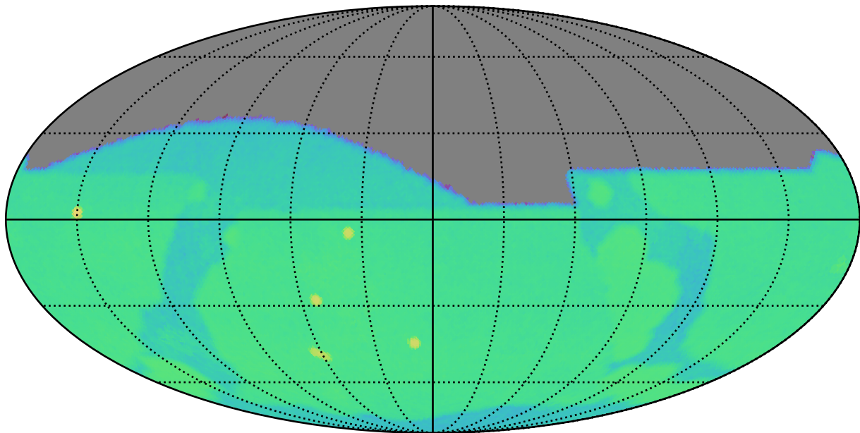
too_combined_s1.0_v3.4_10yrs g: SurfaceBrightLimit
