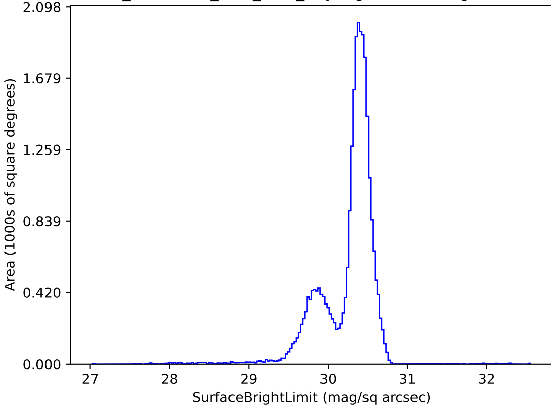
too_combined_s1.0_v3.4_10yrs g: SurfaceBrightLimit
