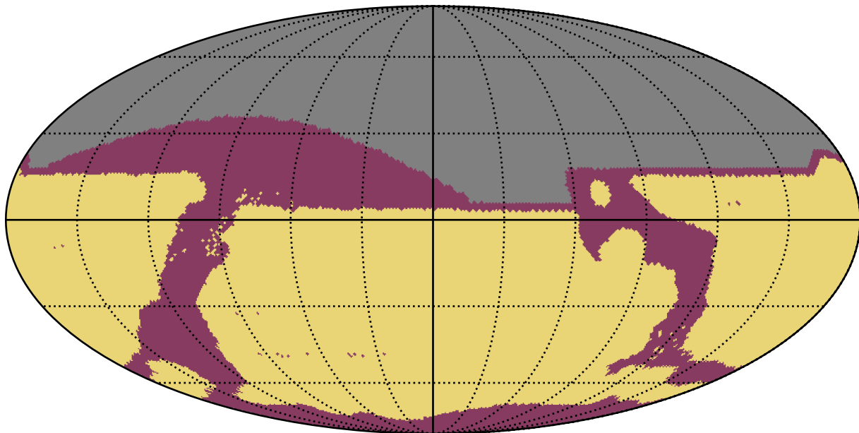
too_combined_s1.0_v3.4_10yrs : RapidRevisits
