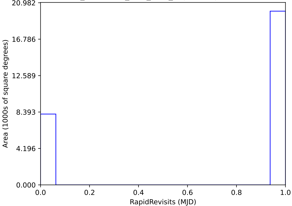
too_combined_s1.0_v3.4_10yrs : RapidRevisits
