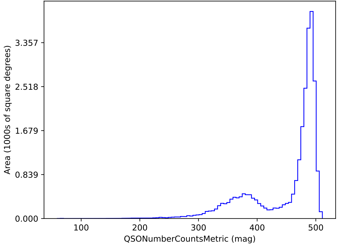
too_combined_s1.0_v3.4_10yrs z band and non-DD: QSONumberCountsMetric
