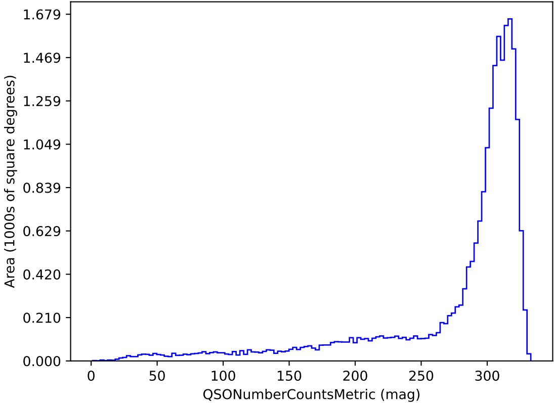
too_combined_s1.0_v3.4_10yrs u band and non-DD: QSONumberCountsMetric
