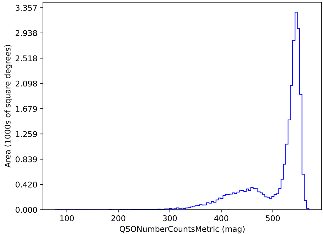
too_combined_s1.0_v3.4_10yrs i band and non-DD: QSONumberCountsMetric
