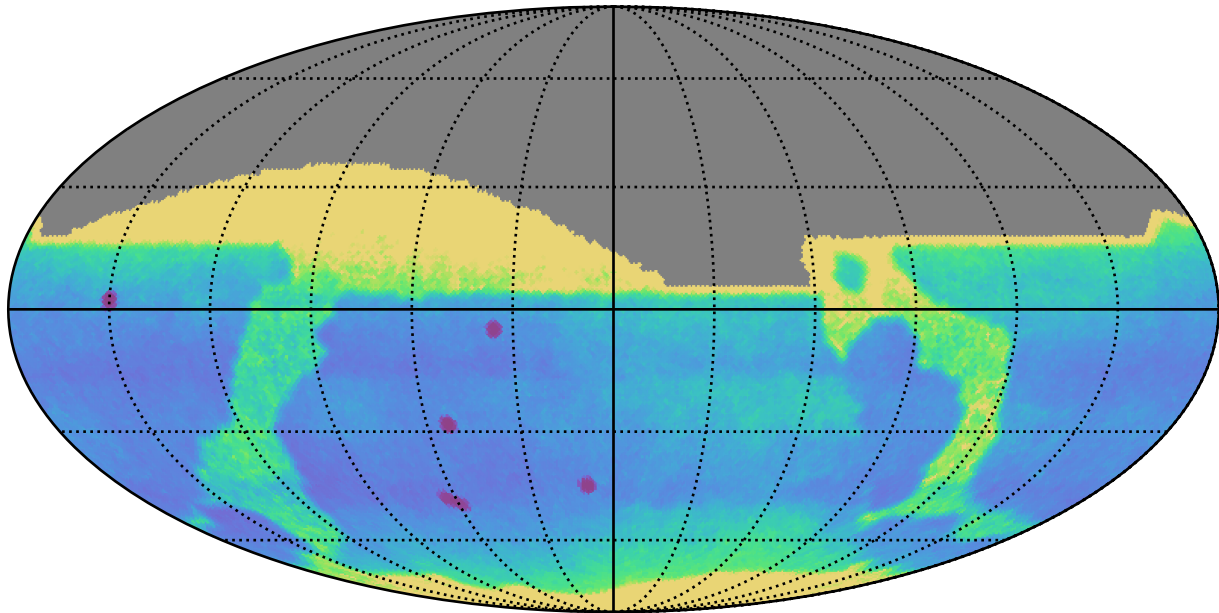
too_combined_s1.0_v3.4_10yrs : Proper Motion Uncert @ 24.0
