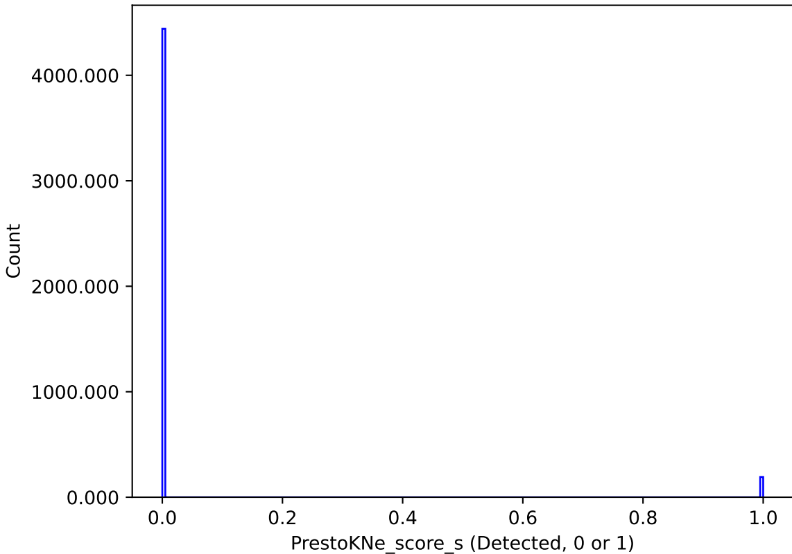
too_combined_s1.0_v3.4_10yrs : PrestoKNe_score_s
