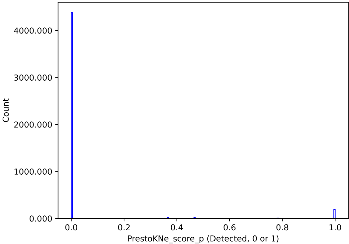
too_combined_s1.0_v3.4_10yrs : PrestoKNe_score_p
