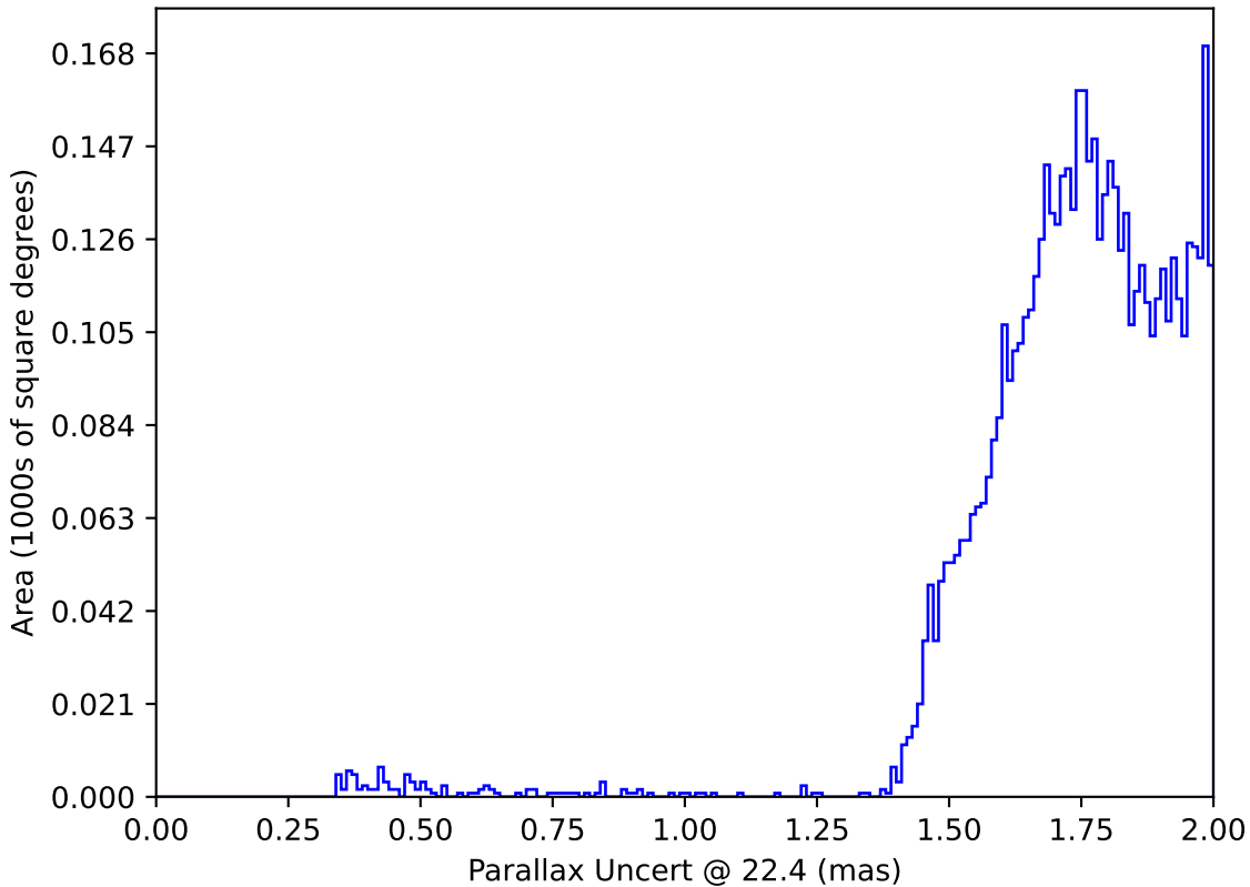
too_combined_s1.0_v3.4_10yrs : Parallax Uncert @ 22.4
