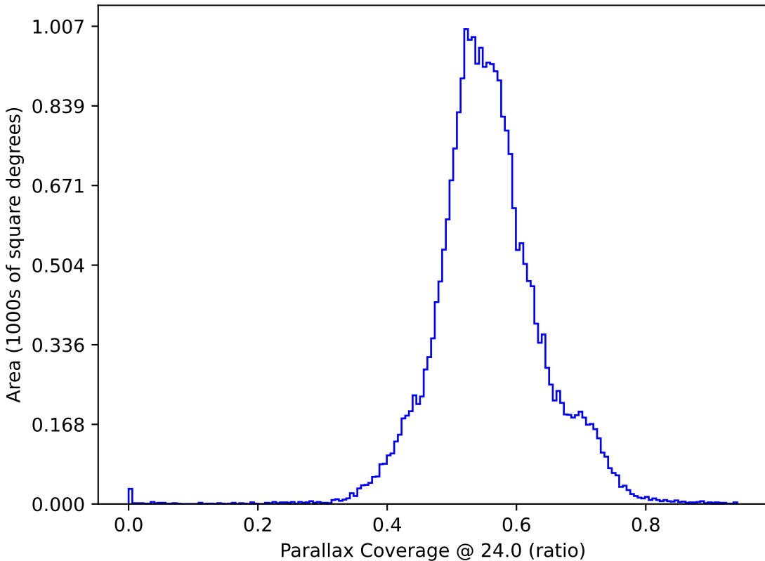
too_combined_s1.0_v3.4_10yrs : Parallax Coverage @ 24.0
