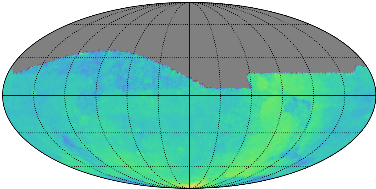
too_combined_s1.0_v3.4_10yrs : Parallax Coverage @ 22.4
